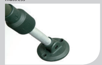
Twist-Lok Leg - simply twist the mechanism on the leg with one hand for instant and infinite adjustment
